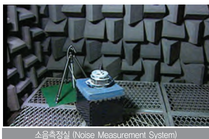
소음측정실 (Noise Measurement System)
